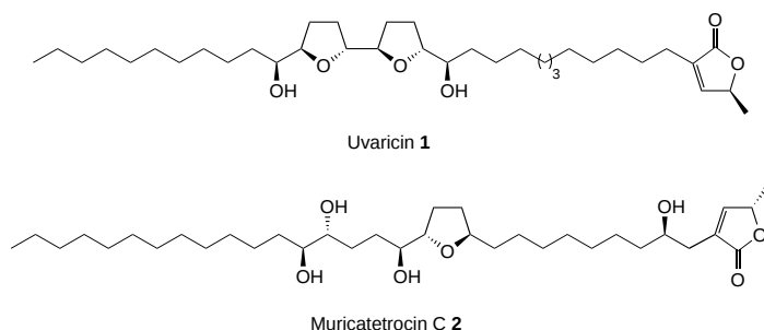
Figure 1. Uvaricin ( 1 ) and muricatetrocin C ( 2 ).
