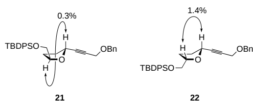
Figure 3. NOE values to confirm the stereochemical outcome of the O – C rearrangement reaction.
