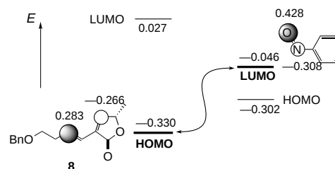
Figure 4. Results of the frontier orbital calculations.
