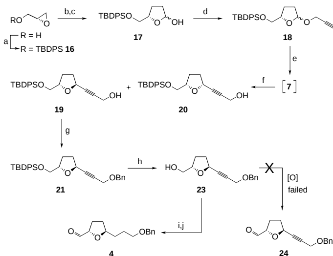
Scheme 4. Synthesis of tetrahydrofuran 4 . a) TBDPSCl, \text{NEt}_3 , DMAP, \text{CH}_2\text{Cl}_2 , rt, 24 h (85 %); b) allylMgBr, \text{CuLi}_2\text{Cl}_4 , (10 mol %), THF, -30^{\circ}\text{C} 2 h (89 %); c) \text{O}_3 , \text{CH}_2\text{Cl}_2 , -78^{\circ}\text{C} , 20 min; \text{PPh}_3 , -78^{\circ}\text{C} \rightarrow \text{rt} , 14 h (93 %); d) prop-2-yn-1-ol, Amberlyst A-15, benzene, reflux, 15 min (91 %); e) n -BuLi, THF, -78^{\circ}\text{C} , 30 min; \text{Bu}_3\text{SnCl} , -78^{\circ}\text{C} \rightarrow \text{rt} , 30 min; f) \text{BF}_3 \cdot \text{OEt}_2 , \text{CH}_2\text{Cl}_2 , -10^{\circ}\text{C} , 10 min [85 %, two steps (5.5:1, 19/20 )]; g) KHMDS, -78^{\circ}\text{C} , 30 min, then BnBr, THF, -78^{\circ}\text{C} \rightarrow \text{rt} (78 %); h) TBAF, THF, rt, 3 h (95 %); i) Raney nickel, \text{H}_2 , EtOH; rt, 30 min (70 %); j) DMSO, (\text{COCl})_2 , \text{CH}_2\text{Cl}_2 , -78^{\circ}\text{C} ; \text{NEt}_3 , -78 \rightarrow \text{rt} (used crude). TBDPSCl = tert -butyldiphenylsilylchloride, DMAP = dimethylaminopyridine, KHMDS = potassium hexamethyldisilazide.
