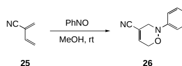
Scheme 6. Reaction of nitrosobenzene with 2-cyanobutadiene ( 25 ).
