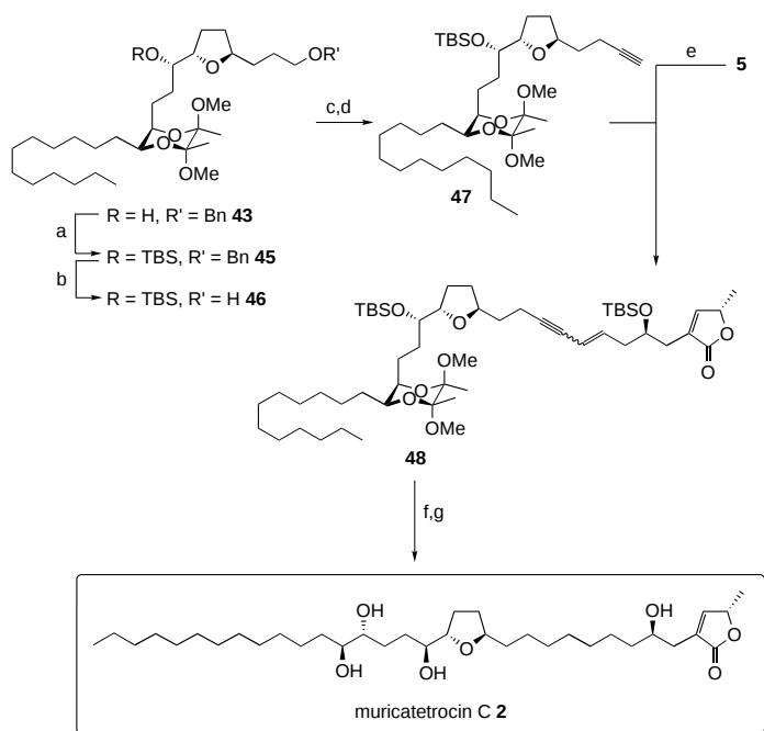
Scheme 10. Second coupling reaction and final steps. a) TBSCl, DMF, imidazole, 45 °C, 14 h (87 %); b) Pd(OH)_2 (20 mol %), H_2 , EtOH; rt, 12 h (94 %); c) DMP, py, CH_2Cl_2 , 0 °C \rightarrow rt, 45 min (96 %); d) diethyl(diazo-methyl)phosphonate, tBuOK , THF, –78 °C, 16 h; then rt, 4 h (76 %); e) [(PPh_3)_2PdCl_2] (10 mol %), CuI (30 mol %), NEt_3 , rt, 3 h (81 %); f) [Rh(PPh_3)_3Cl] , H_2 , benzene/EtOH 1:1, rt, 11 h (76 %); g) TFA/ H_2O 9:1, rt, 30 s; repeat (82 %). DMP = Dess–Martin periodinane, TFA = trifluoroacetic acid.
