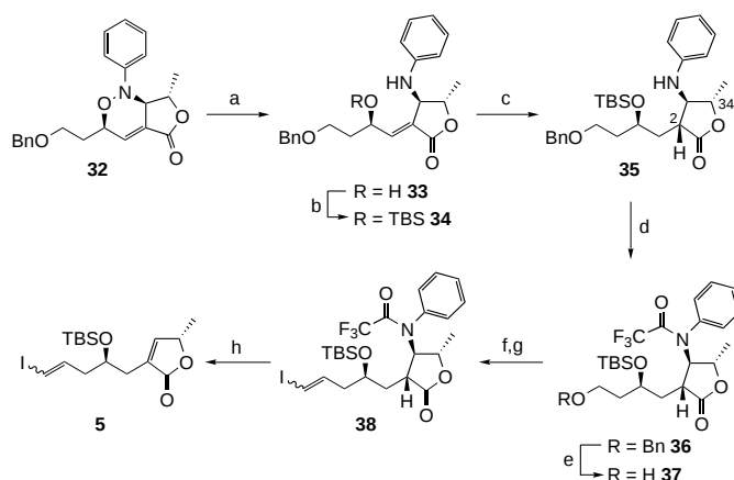
Scheme 8. Synthesis of the butenolide fragment 5 . a) [Mo(CO) 6 ], MeCN, reflux, 4 h; then 32 , H 2 O, rt, 15 min (70 %); b) TBSCl, imidazole, DMF, rt, 14 h (83 %); c) PtO 2 (33 mol %), H 2 , MeOH; rt, 90 min (98 %); d) TFAA, Hünig's base, CH 2 Cl 2 , 0 °C, 30 min; e) Pd(OH) 2 (20 mol %), H 2 , MeOH; rt, 48 h (90 % two steps); f) DMSO, (COCl) 2 , CH 2 Cl 2 , –78 °C; NEt 3 , –78 °C → 0 °C; g) CrCl 2 , CHI 3 , THF, 0 °C → rt, 14 h (80 % two steps, E/Z 4:1); h) DBU, CH 2 Cl 2 , 0 °C, 60 min (91 %). TFAA = trifluoroacetic anhydride, DBU = 1,8-diazabicyclo[5.4.0]undec-7-ene.
