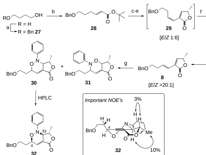
Scheme 7. Synthesis of the hetero-Diels–Alder adduct 32 . a) NaH; BnBr, DMF, 0 °C (82 %); b) DMSO, (COCl) 2 , CH 2 Cl 2 , –78 °C; NEt 3 , –78 → rt, then ( tert -butoxycarbonylmethylene)triphenylphosphorane, CH 2 Cl 2 , 0 °C → rt, 14 h (96 %); c) LDA/HMPA/THF, –78 °C, 30 min, then ( S )-2-( tert -butyldimethylsilyloxy)propanal, –78 → 0 °C; d) MeOH/HCl (sat.), rt, 5 min, (repeat); e) MsCl, NEt 3 , CH 2 Cl 2 , 0 °C, 30 min ( E/Z 1:6); f) I 2 (5 mol %), sunlamp irradiation, rt, 4 h (56 %, four steps; E/Z , >20:1); g) PhNO, MeOH/CH 2 Cl 2 (1:1), 0 °C, 21 h [91 % ( 30/31 7:3)]; DMF = N,N -dimethylformamide, LDA = lithium diisopropylamide, HMPA = hexamethyl phosphoramide, MsCl = methanesulfonyl chloride.
