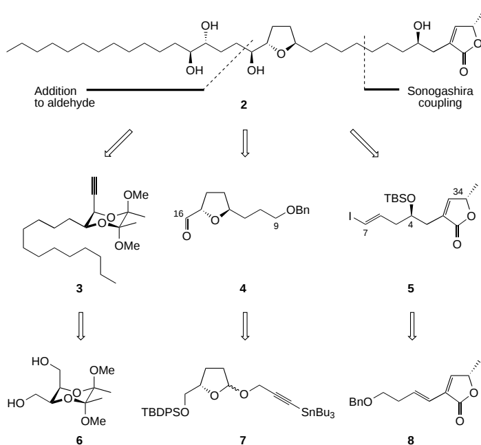
Scheme 1. Synthetic plan for 2 . Bn = benzyl, TBS = tert -butyldimethylsilyl, TBDPS = tert -butyldiphenylsilyl.
