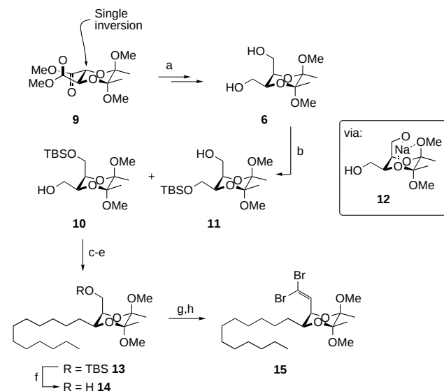
Scheme 2. Synthesis of gem -dibromo olefin 15 . a) ref. [21]; b) NaH; THF/pentane, 0 °C → rt, 30 min, then TBSCl, 40 min (72 %); c) DMSO, (COCl) 2 , CH 2 Cl 2 , –78 °C; NEt 3 , –78 → rt; d) CH 3 (CH 2 ) 10 PPh 3 I, n -BuLi, THF, –78 °C, 30 min (92 %, two steps; Z/E 8:1); e) Raney nickel, H 2 , EtOH; rt, 30 min (90 %); f) TBAF, THF, rt, 2 h; g) DMSO, (COCl) 2 , CH 2 Cl 2 , –78 °C; NEt 3 , –78 → 0 °C; h) PPh 3 , CBr 4 , CH 2 Cl 2 , 0 °C, 30 min, (88 %, three steps). TBAF = tetra- n -butylammonium fluoride, TBSCl = tert -butyldimethylsilyl chloride.
