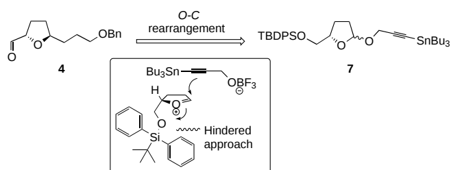
Scheme 3. Synthetic plan towards tetrahydrofuran 4 .
