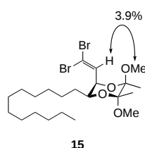
Figure 2. NOE to confirm axial disposition of the gem -dibromo olefin 15 .
