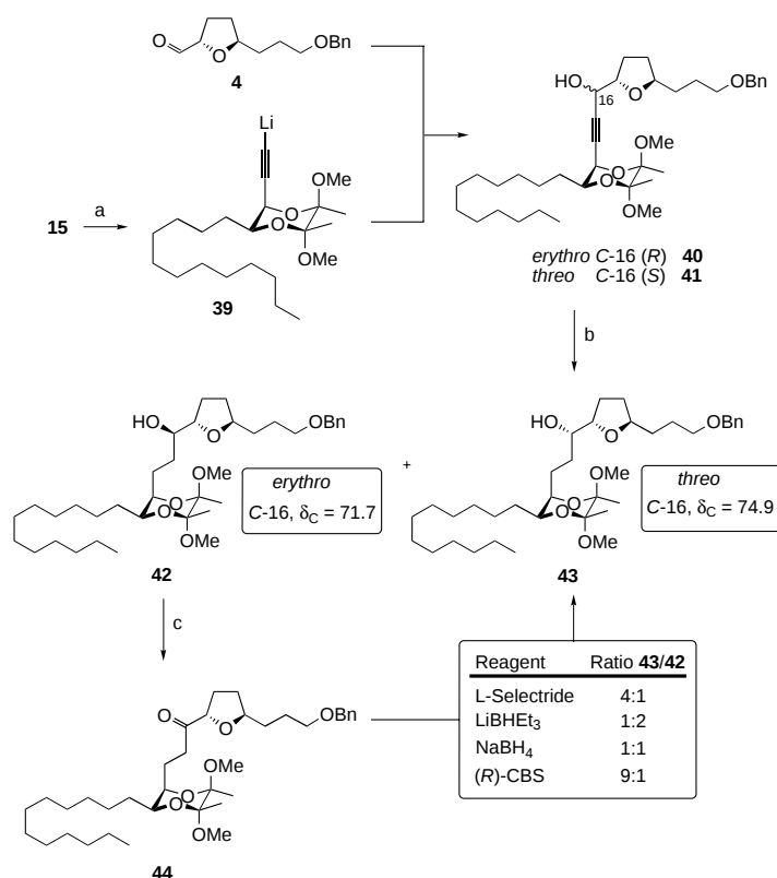
Scheme 9. Coupling fragments 39 and 4 . a) n -BuLi, THF, -78 \rightarrow 0^{\circ}\text{C} , 30 min; -78^{\circ}\text{C} then 4 (63 % two steps; 40/41 , 1.8:1); b) Raney nickel, \text{H}_2 , EtOH; rt, 60 min ( 43 18 %, 42+43 71 %); c) DMSO, (\text{COCl})_2 , \text{CH}_2\text{Cl}_2 , -78^{\circ}\text{C} ; \text{NEt}_3 , -78 \rightarrow \text{rt} (80 %).
