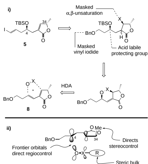
Scheme 5. i) Synthetic plan towards fragment 5 ; ii) requirements of the dienophile for the successful induction of stereochemistry.
